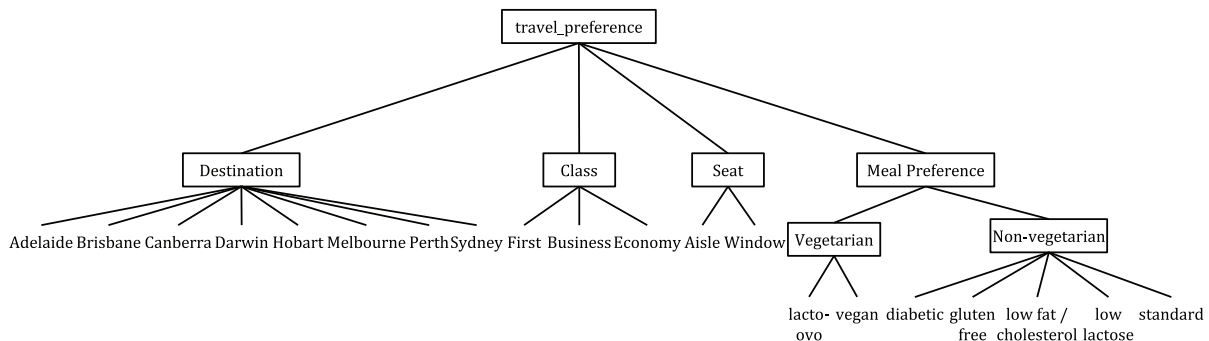
Figure B.4 — Classification tree example
